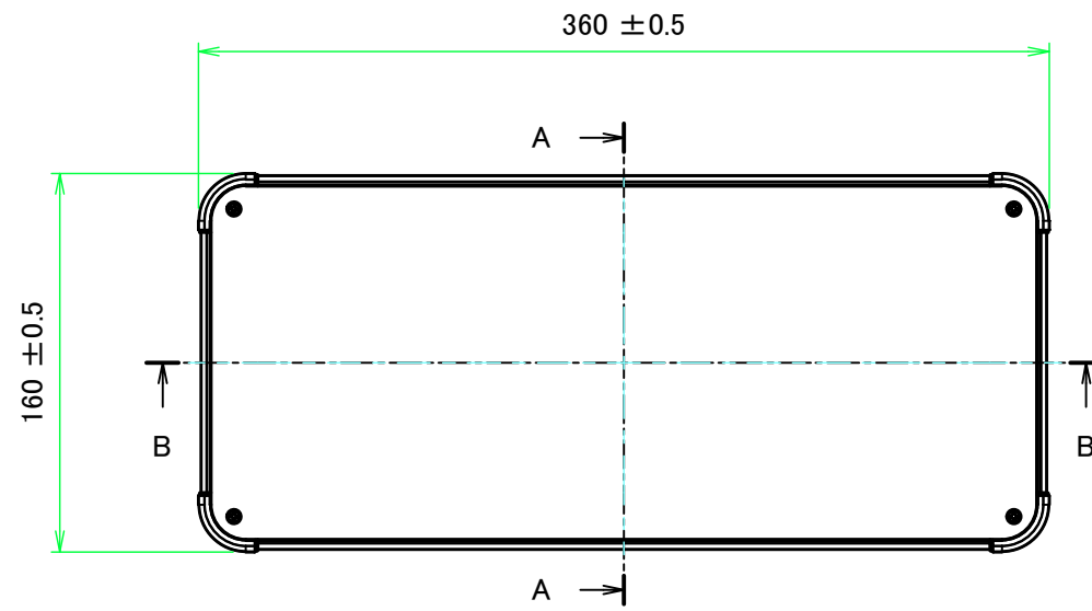
E view
